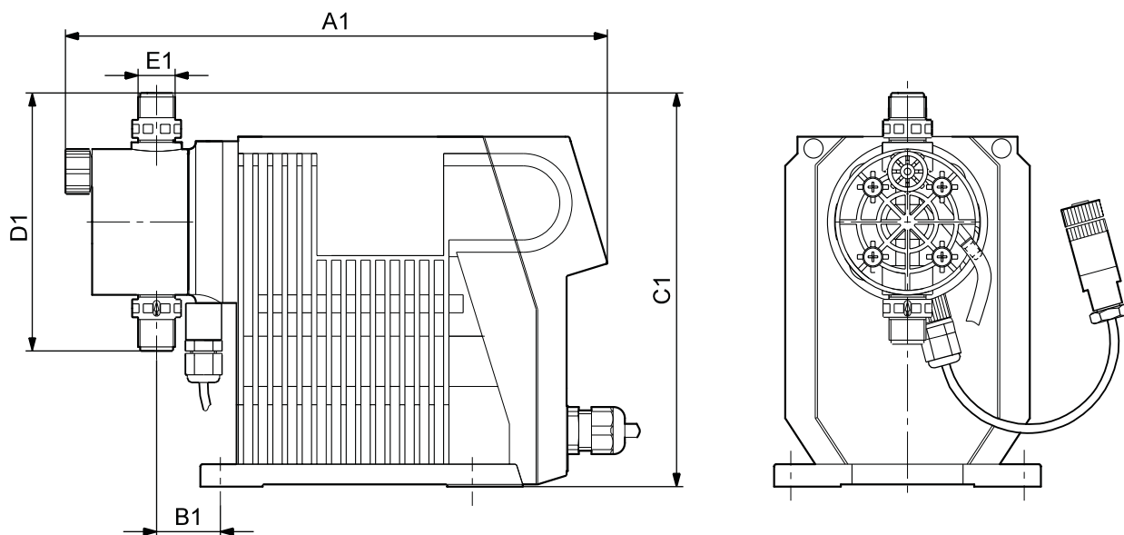
Fig. 3 DDI 209 AR with leak detection
