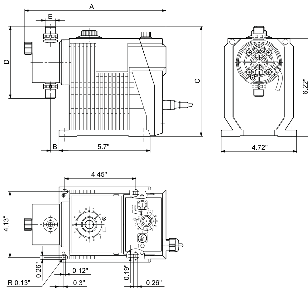
Fig. 14 Dimensions, DMI
