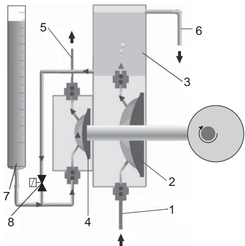
Fig. 13 Functional principle of the Plus 3 system
